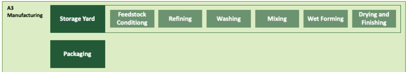
Figure 2. Cellulosic Fiberboard manufacturing process
